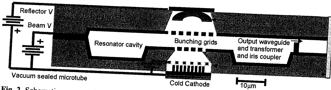
Fig. 2. Schematic cross section of proposed nanoklystron. The cathode is composed of a carbon nanotube field emitter array (Fig. 7) with a built-in grid. The cavity, beam and output waveguide are etched from two silicon wafers which are later joined by thermocompression bonding. The wiring and grid layers are formed lithographically. The repeller and cathode are drop-in parts and vacuum sealing is performed in the last step.
