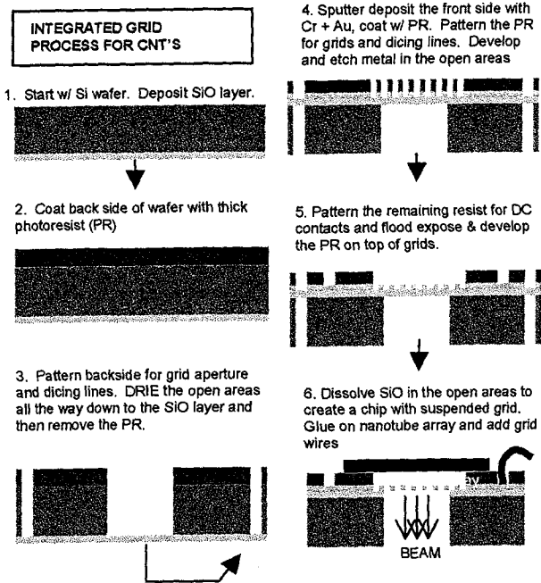
Fig. 9. Steps for fabricating integral grid nanotube cathode.
