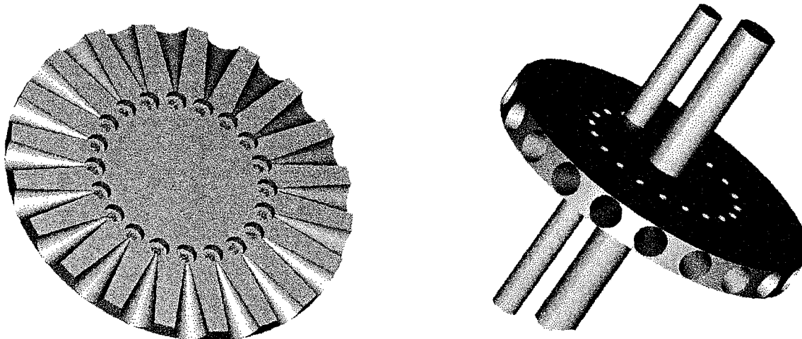
Fig. 10. Left: Possible nanoklystron array for multiple frequency or multiple power output. Right: Frequency switching or redundancy is obtained by mechanical indexing.
